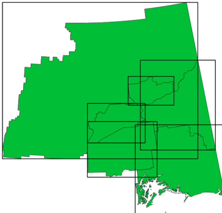
Рис. 28.61: Black lines represent the bounding boxes of each polygon feature
