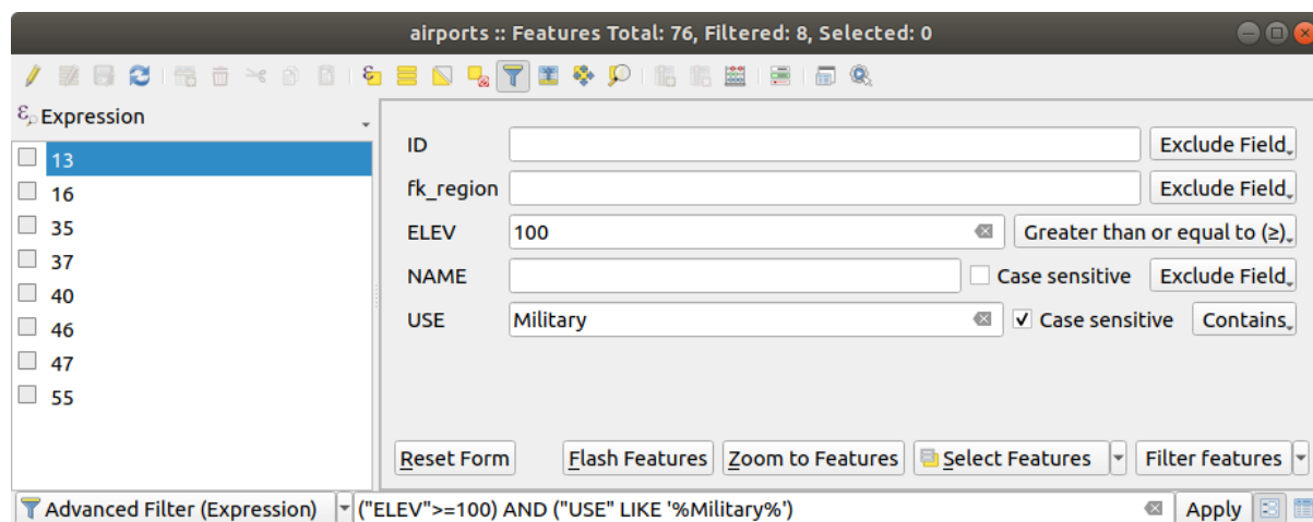
Рис. 16.70: Attribute table filtered by the filter form
