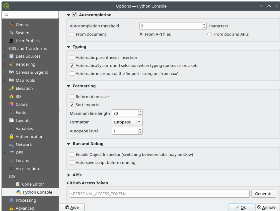
Рис. 9.28: Python Console settings
