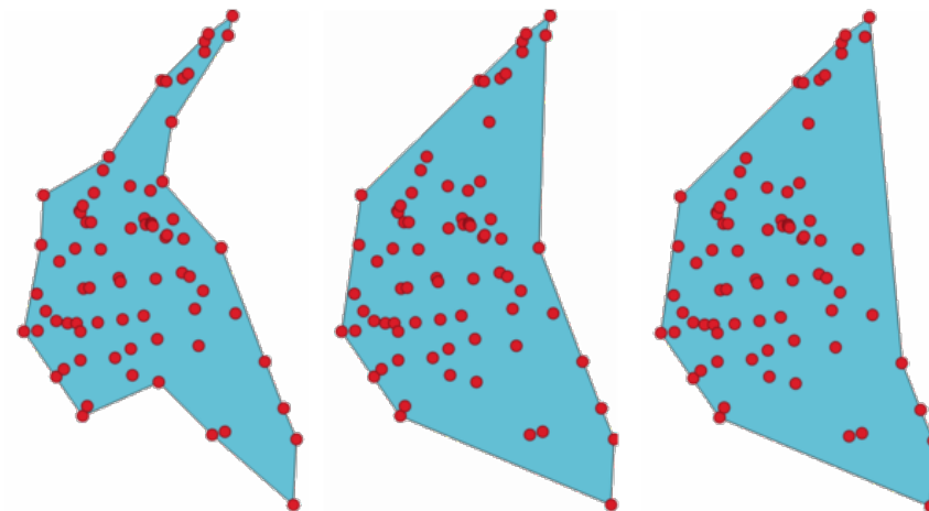
Рис. 28.70: Concave hulls with different thresholds (0.3, 0.6, 0.9)
