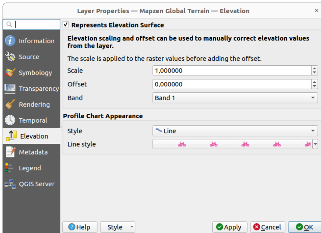
Рис. 17.17: Raster Elevation Properties
