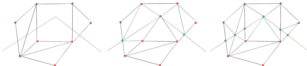
Рис. 18.15: Force Mesh using a line geometry - Results without (middle) and with (right) new vertex on edges intersection
