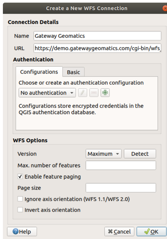
Рис. 23.6: Creating a connection to a WFS server
