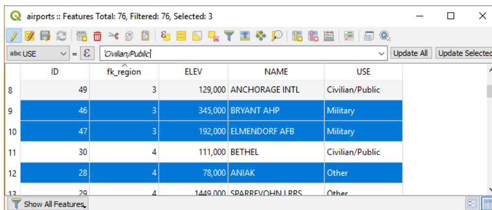
Рис. 16.73: Quick Field Calculation Bar
