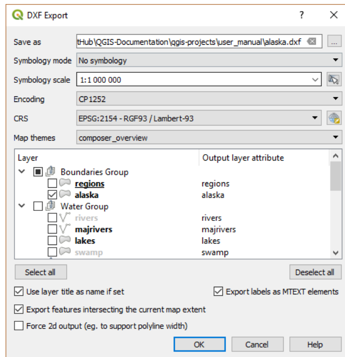
Рис. 15.29: Exporting a project to DXF dialog
