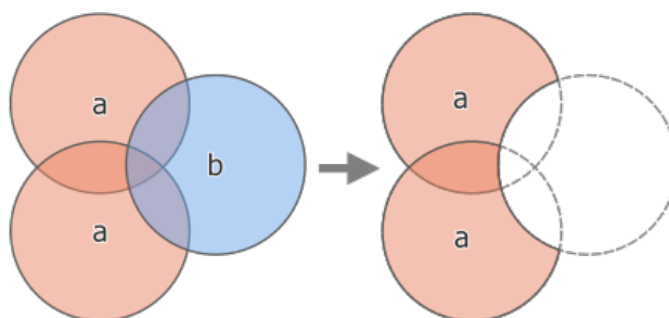
Рис. 28.119: Difference operation between a two-features input layer „a“ and a single feature overlay layer „b“ (left) - resulting in a new layer with the modified „a“ features (right)
