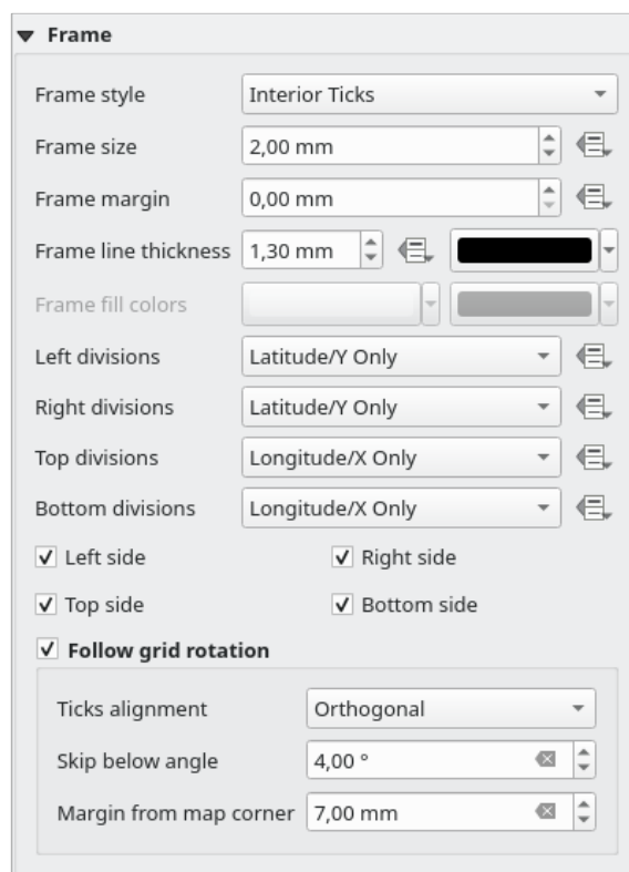
Рис. 22.20: Grid Frame Dialog
