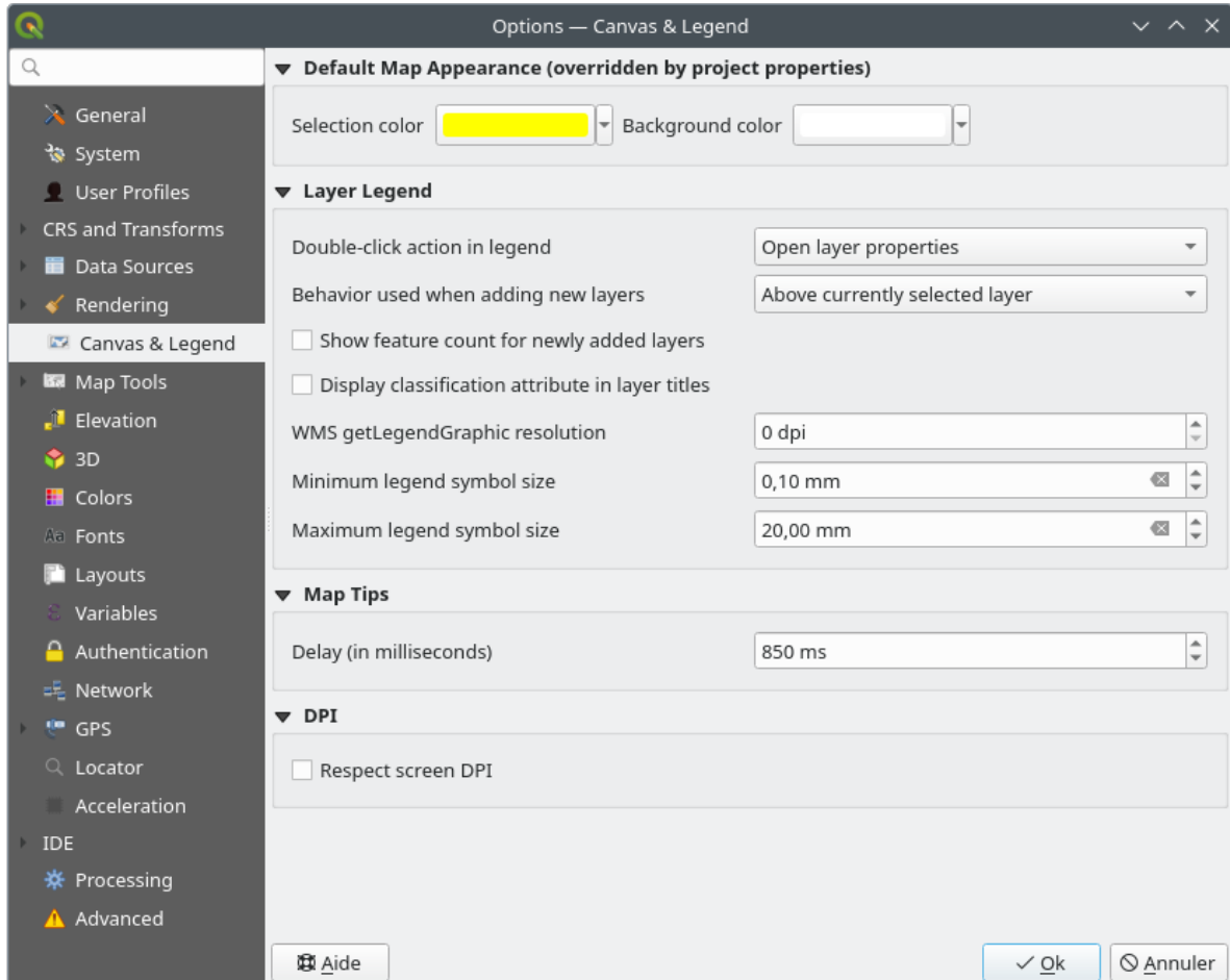
Рис. 9.13: Canvas & Legend settings
