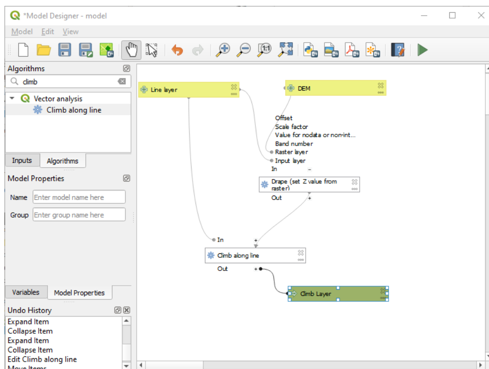
Рис. 27.24: A complete model
