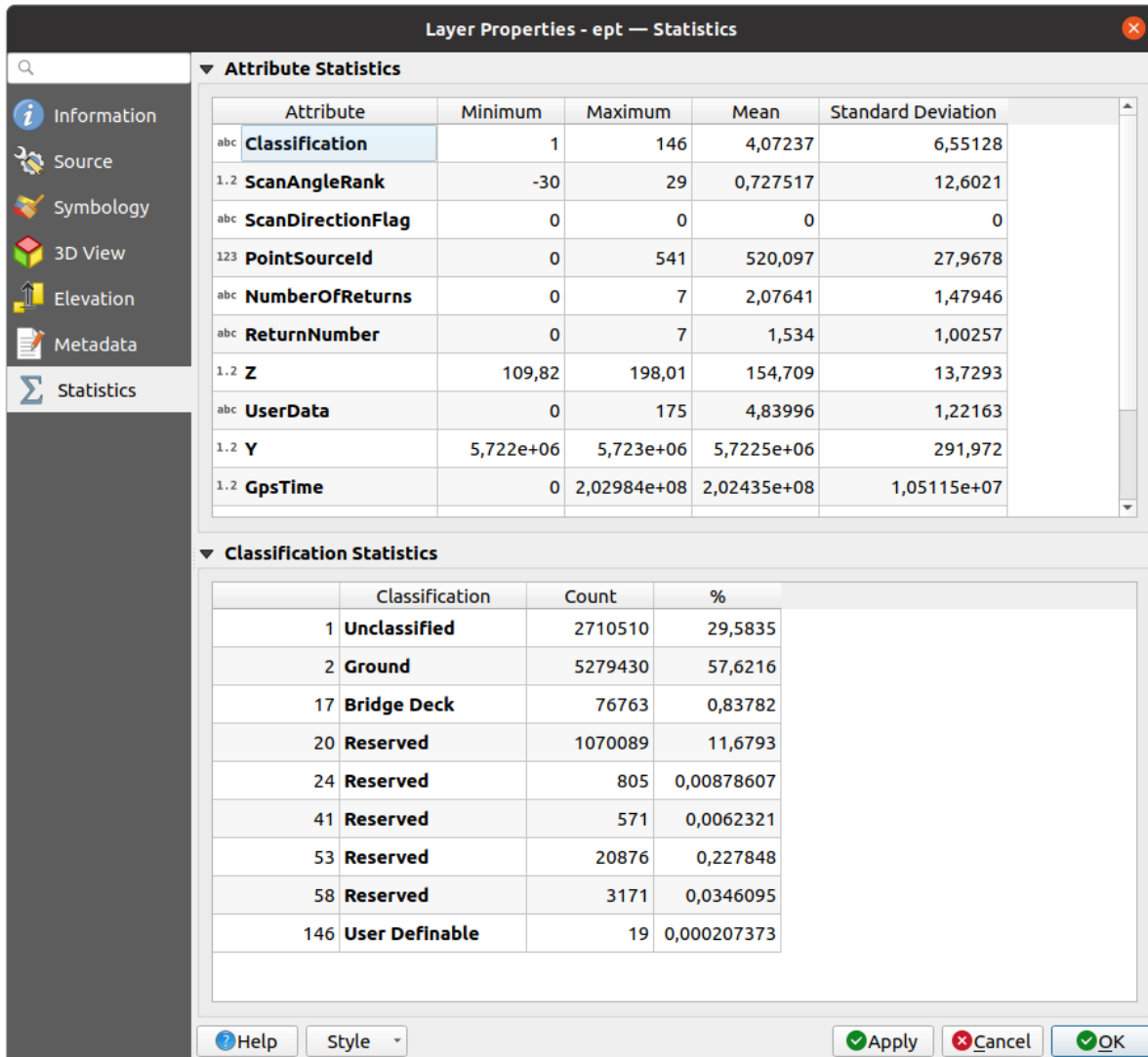
Рис. 20.11: The point cloud statistics tab
