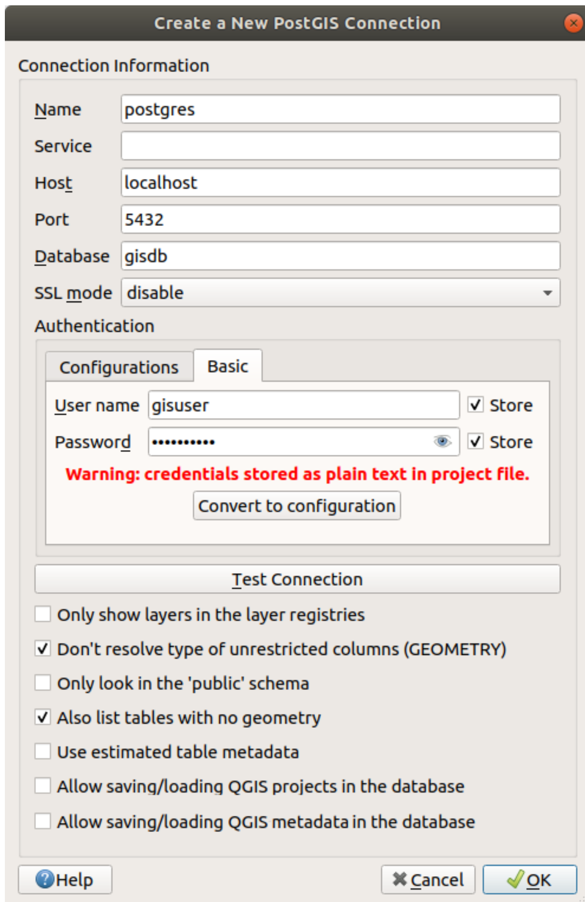
Рис. 15.12: Create a New PostGIS Connection Dialog
