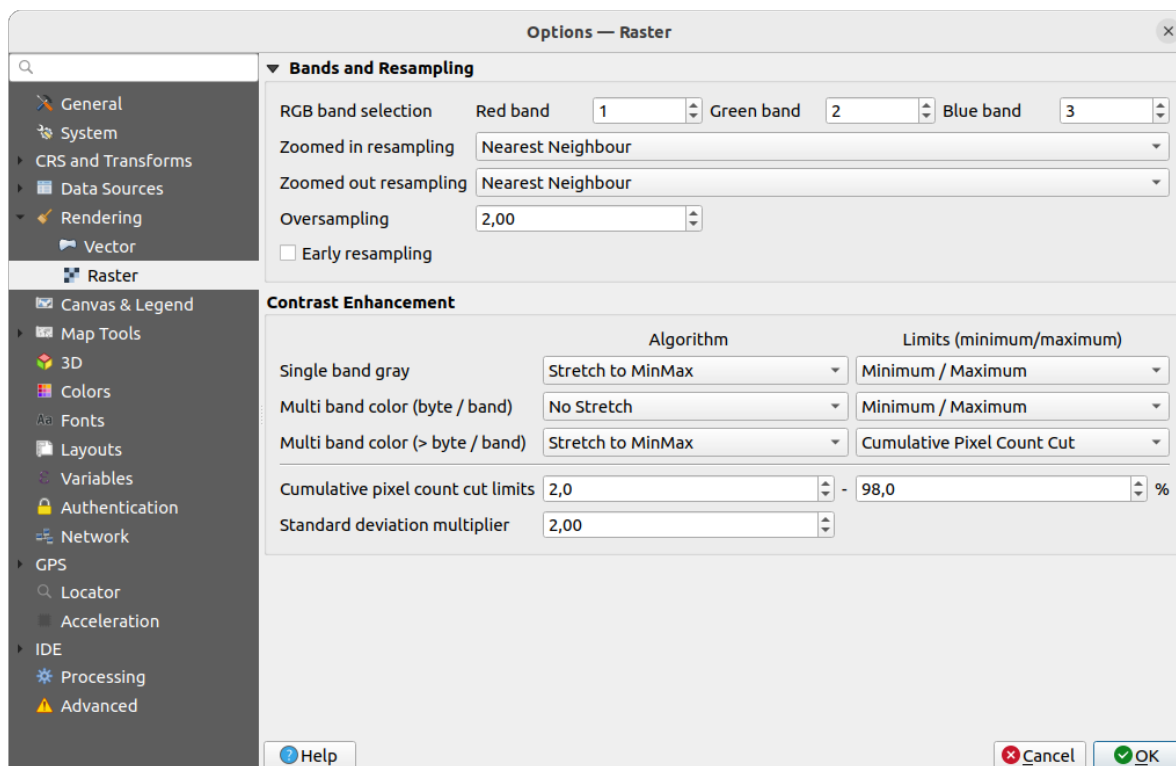
Рис. 9.12: Raster rendering settings
