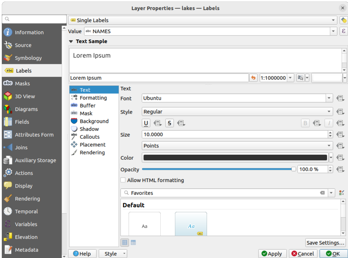
Рис. 5.5: Showing Lakes names
