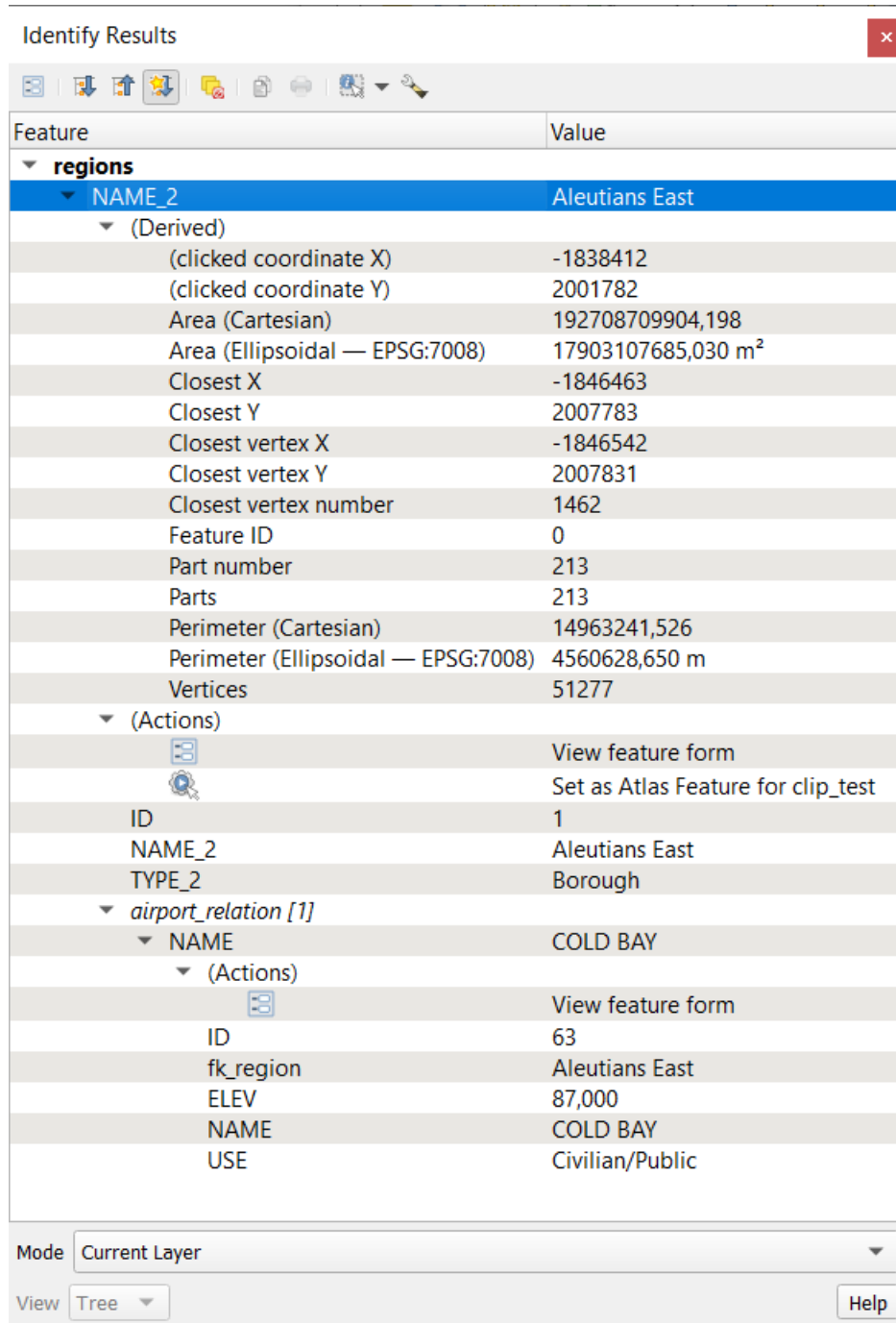
Рис. 12.11: Identify Results dialog
