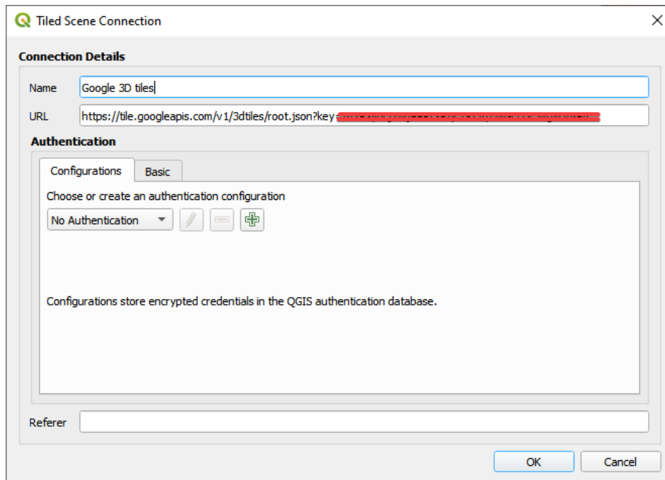
Рис. 21.2: Google 3D Tiles connection
