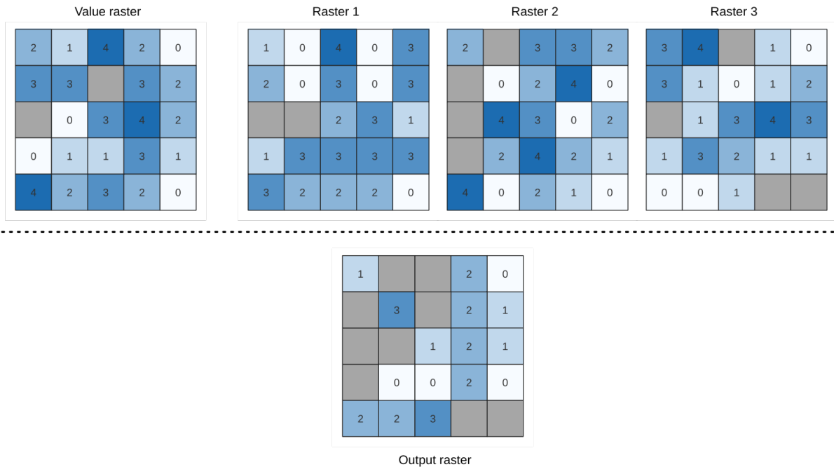
Рис. 28.25: For each cell in the output raster, the value represents the number of times that the corresponding cells in the list of rasters are less than the value raster. NoData cells (grey) are taken into account.
