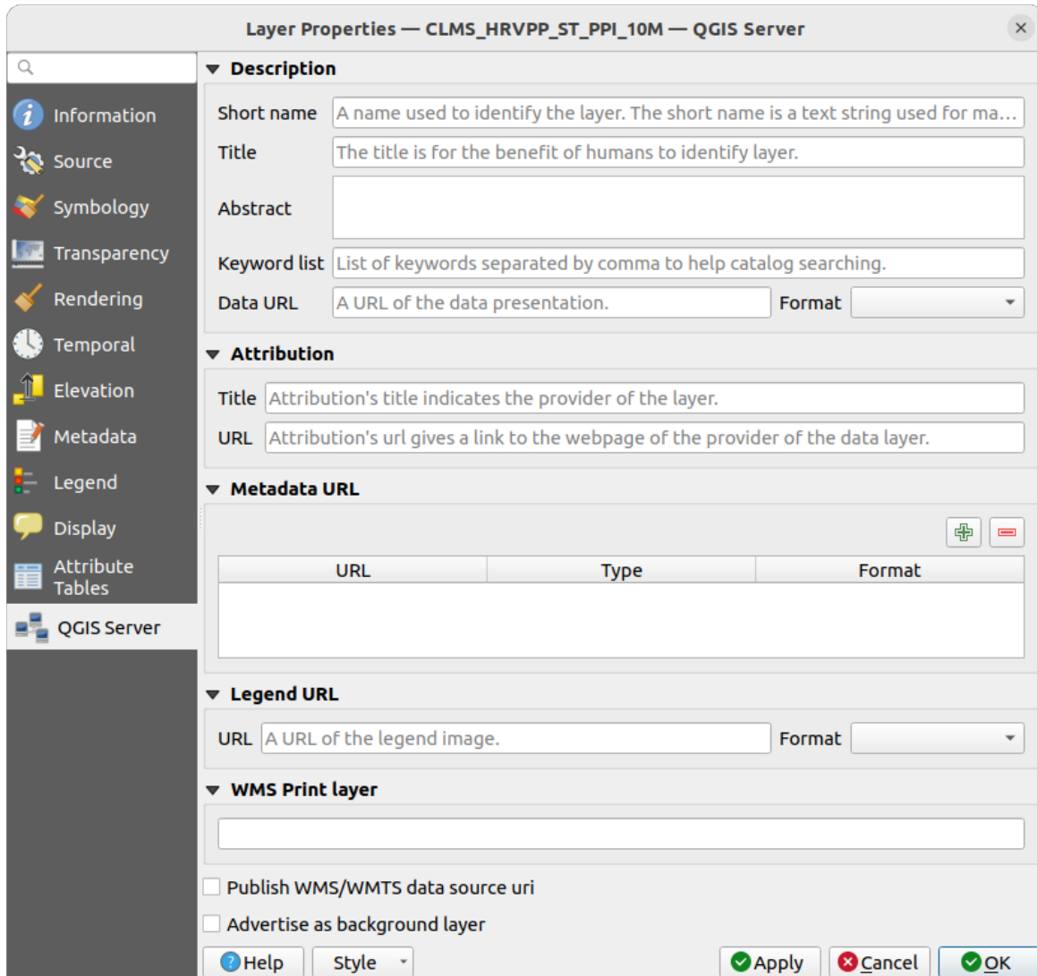
Рис. 23.5: QGIS Server properties of a WMS/WMTS layer
