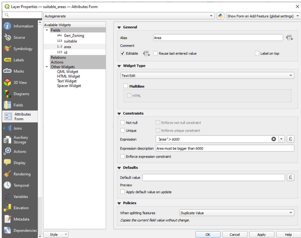
Рис. 16.44: Dialog to select an edit widget for an attribute column
