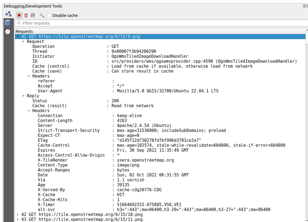
Рис. 12.6: Network Logger output for GET Request
