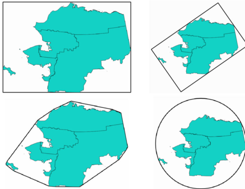
Рис. 28.90: Clockwise from top left: envelope, oriented rectangle, circle, convex hull
