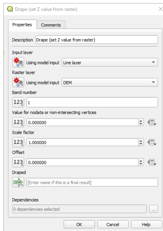
Рис. 27.23: Algorithm Input and Output parameters
