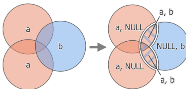
Рис. 28.129: Union operation between a two-feature input layer „a“ and a single feature overlay layer „b“ (left) - resulting five-feature layer with attributes from both layers (right)
