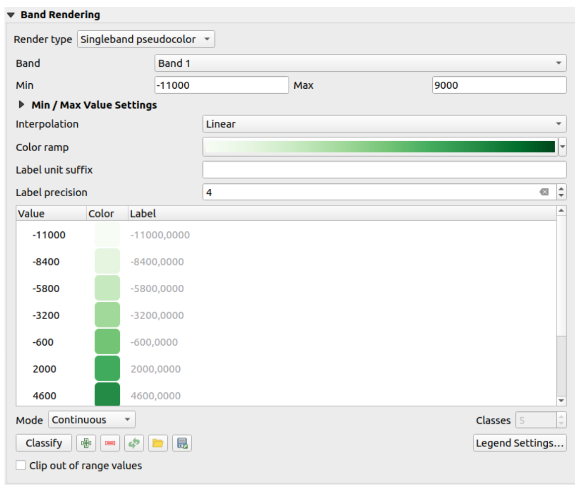
Рис. 17.5: Raster Symbolology - Singleband pseudocolor rendering
