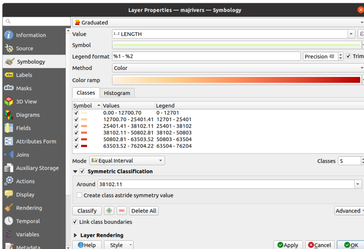
Рис. 16.5: Graduated Symbolizing options
