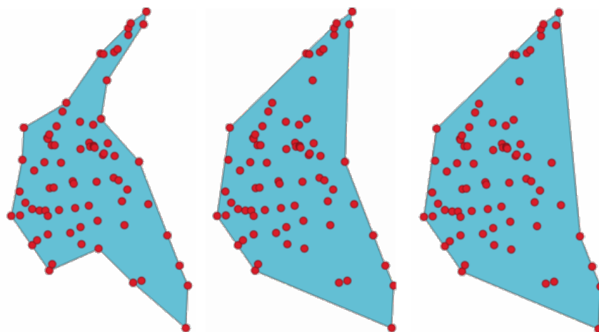
Figura28.70: Concave hulls with different thresholds (0.3, 0.6, 0.9)
