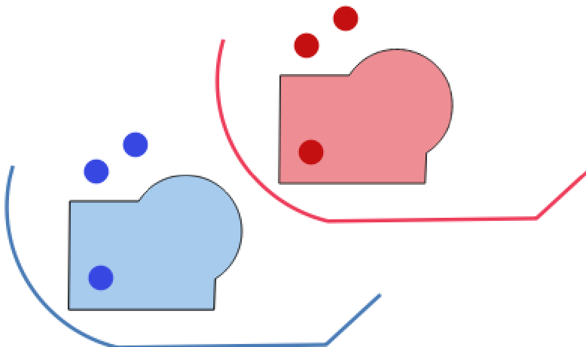
Figura13.9: Translating features
