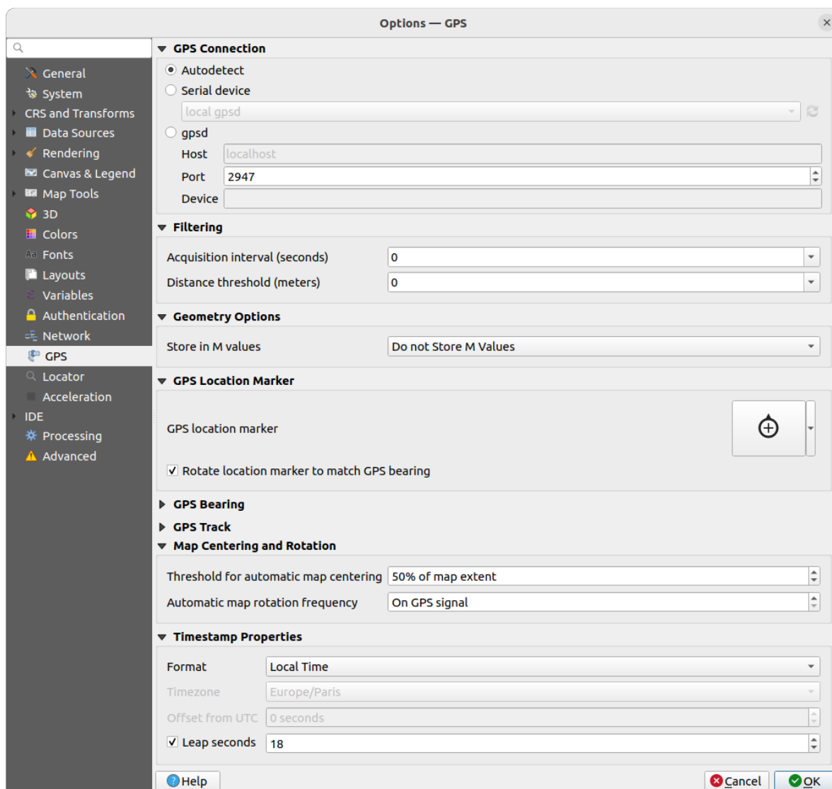
Figura9.24: GPS settings
