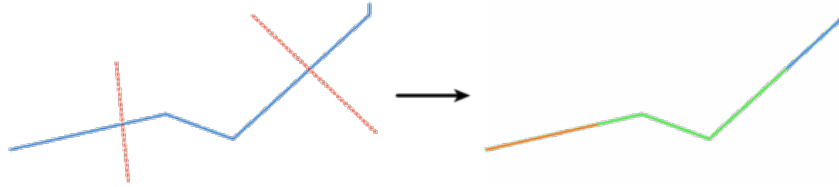
Figura28.126: Split lines
