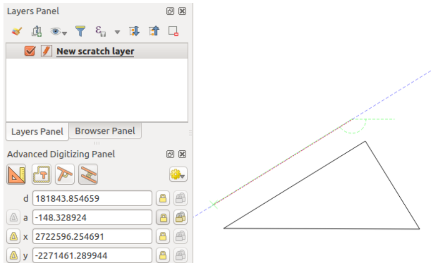
Figura16.94: Parallel digitizing
