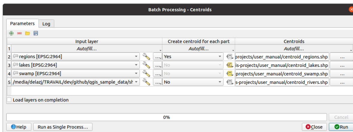
Figura27.34: Batch Processing
