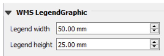
Figura22.32: WMS LegendGraphic
