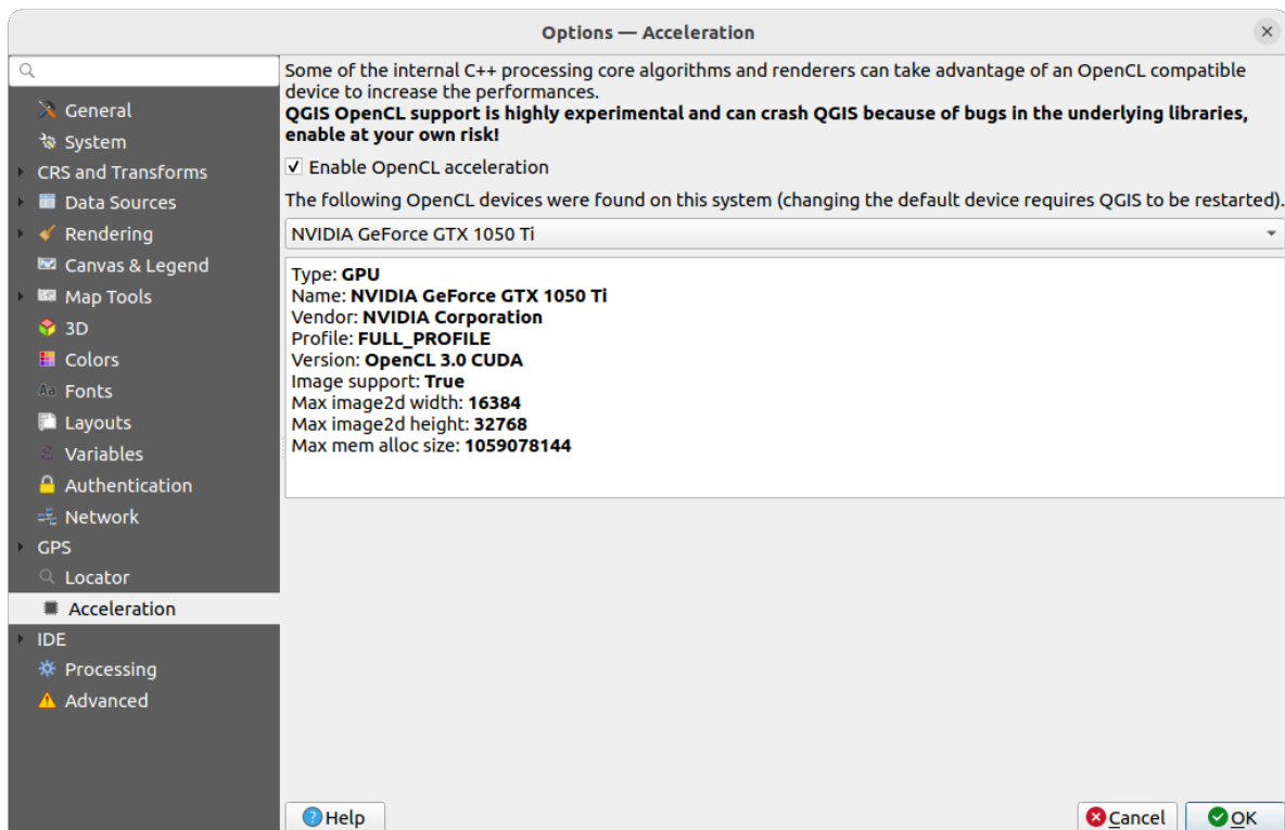
Figura9.26: Acceleration settings
