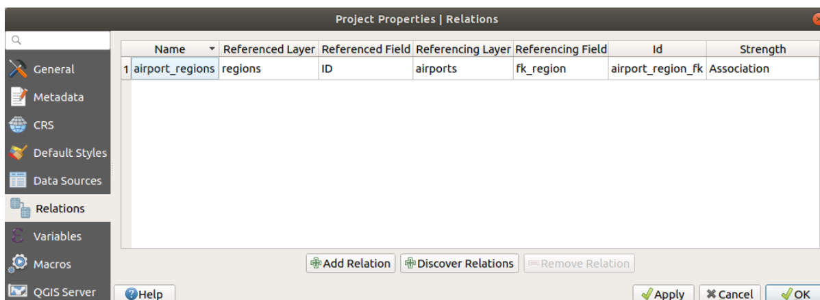
Figura9.36: Relations tab
