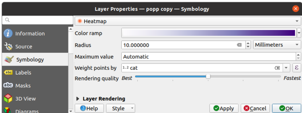
Figura16.11: Heatmap dialog
