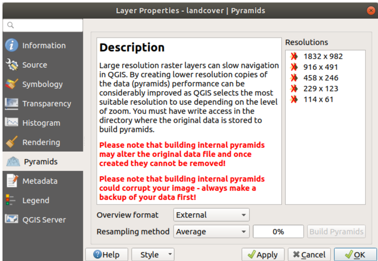
Figura17.16: Raster Pyramids
