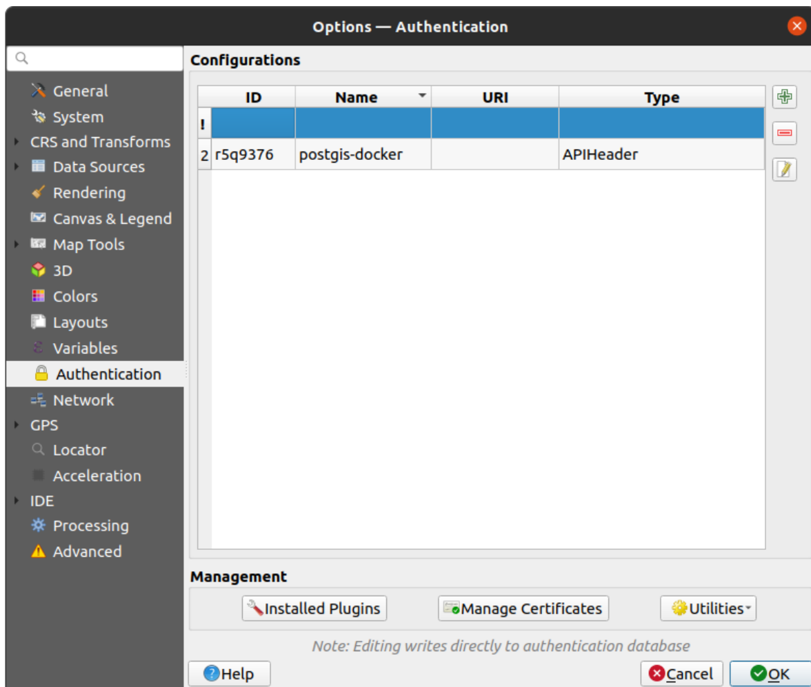
Figura25.5: Configurations editor
