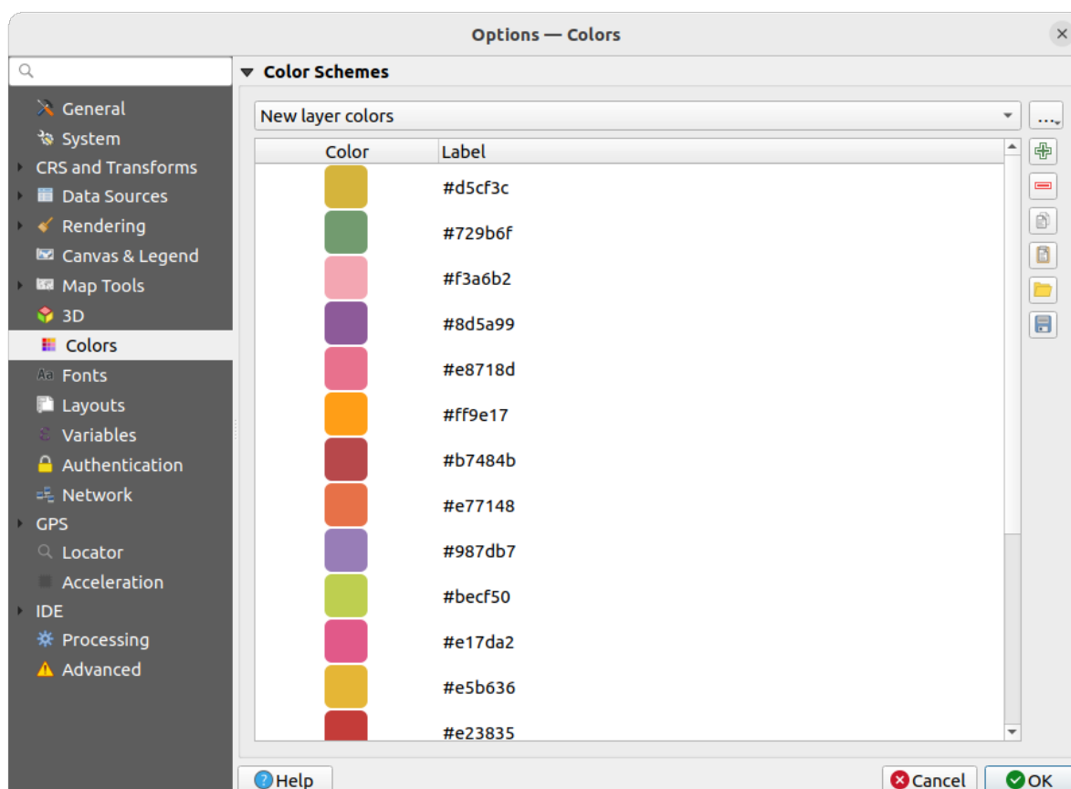
Figura9.18: Colors settings
