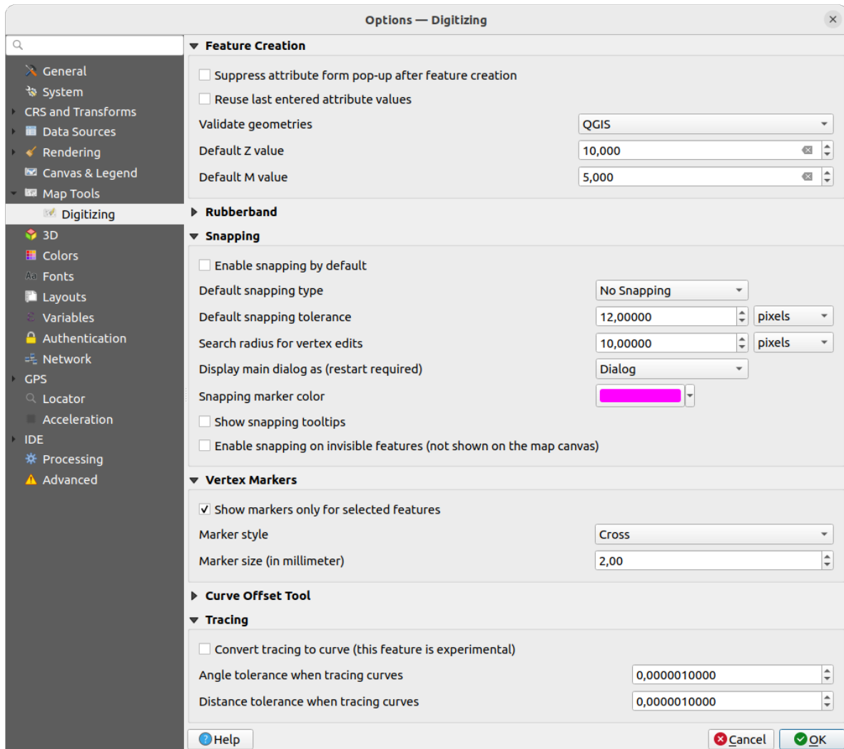
Figura9.15: Digitizing settings
