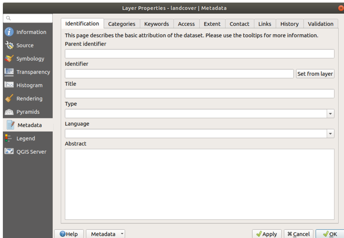
Figura17.18: Raster Metadata
