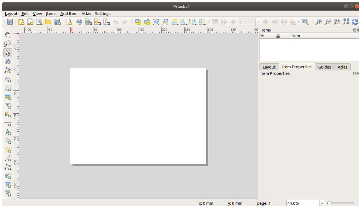
Figura22.2: Print Layout
