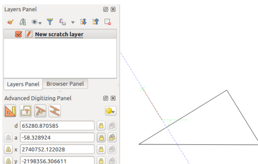
Figura16.93: Perpendicular digitizing
