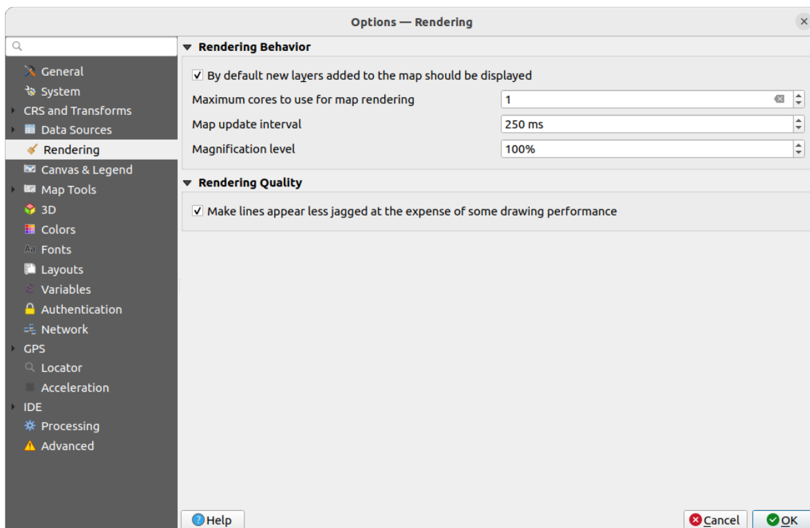
Figura9.10: Rendering settings
