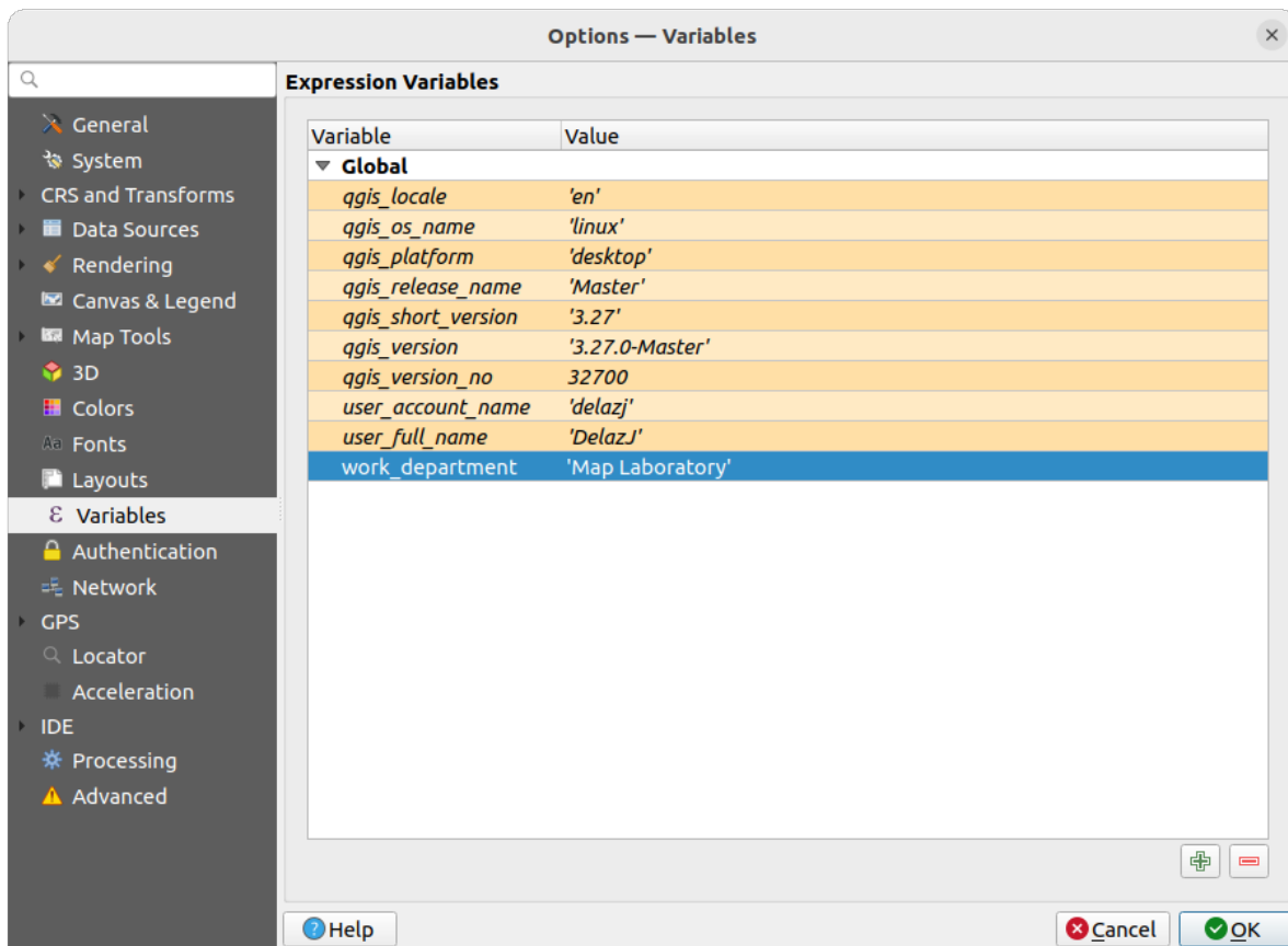
Figura9.21: Variables settings
