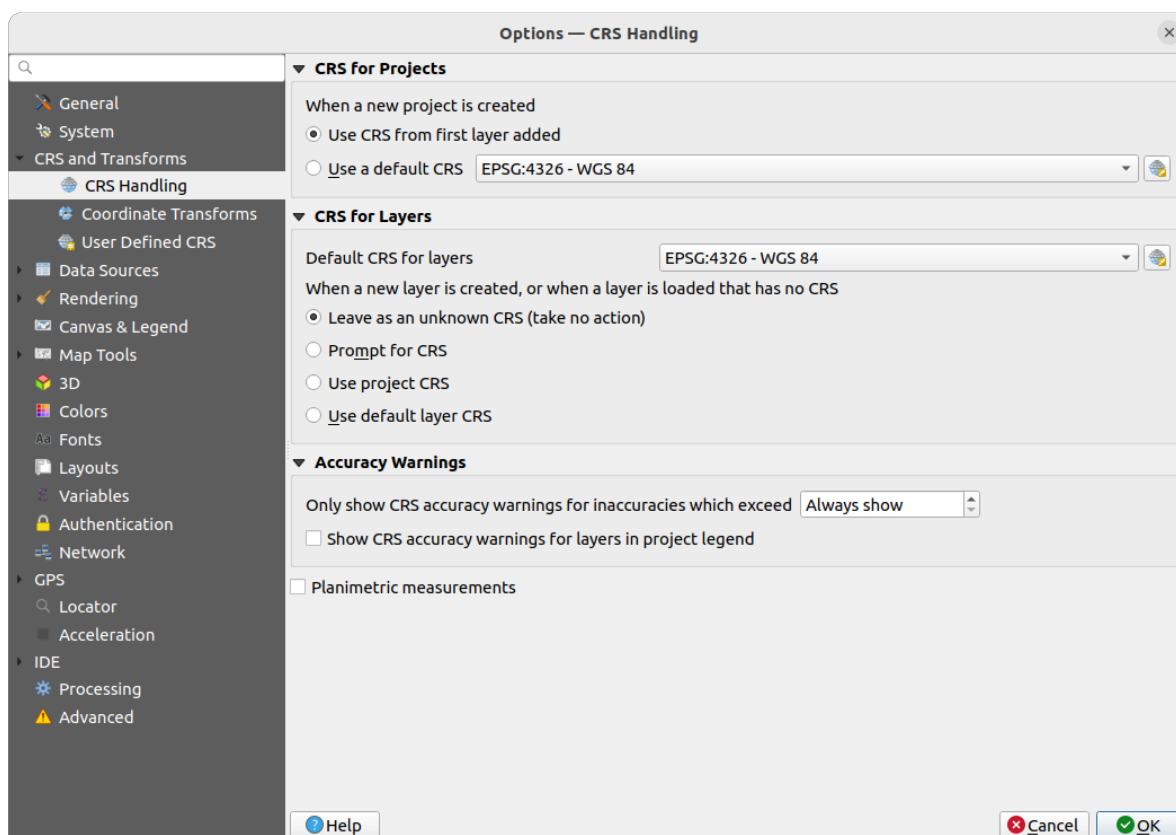
Figura9.3: CRS Settings
