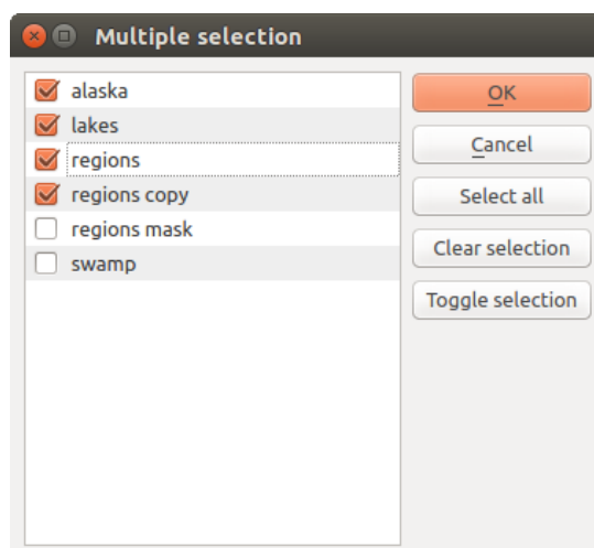
Figura27.14: Multiple Selection
