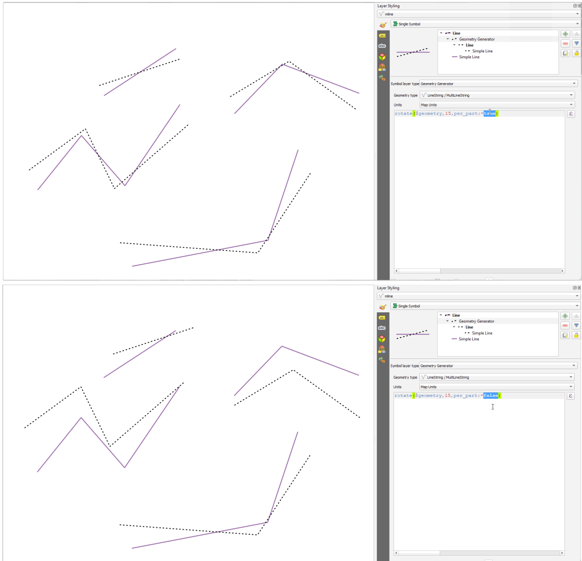
Figura13.7: Rotating features
