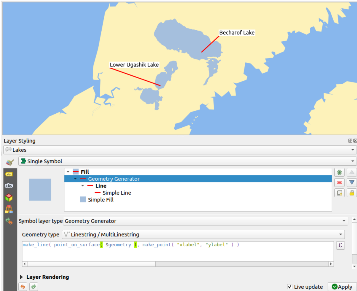
Figura16.33: Moved labels
