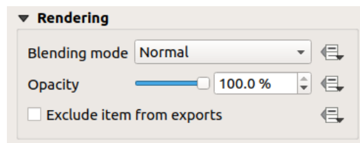
Figura22.13: Rendering mode
