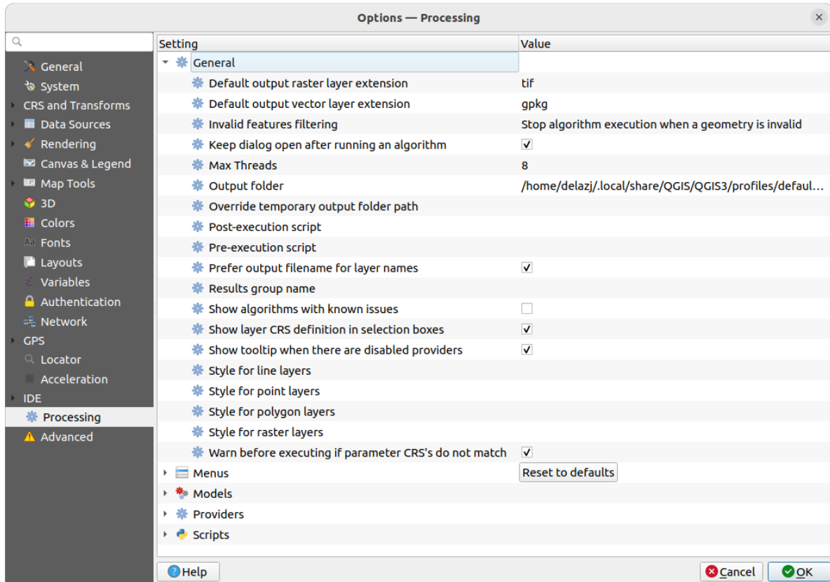
Figura9.29: Processing settings
