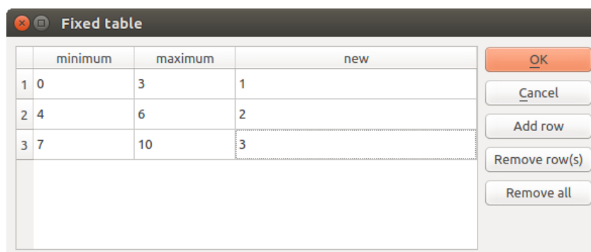
Figura27.15: Fixed Table
