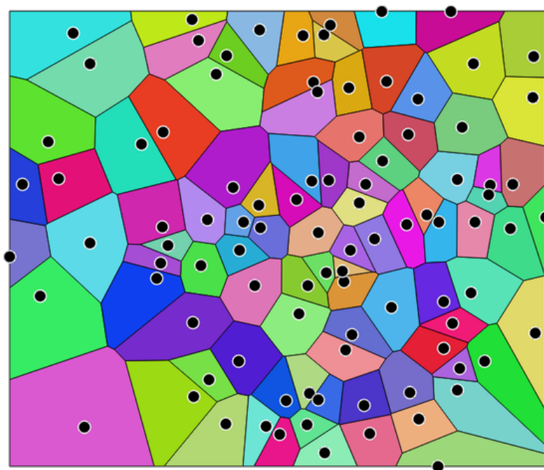
Figura28.117: Voronoi polygons
