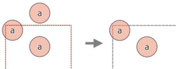
Figura28.121: Extract operation between a three-feature input layer “a” and a dashed extent (left) - resulting features with dashed extent for reference (right)
