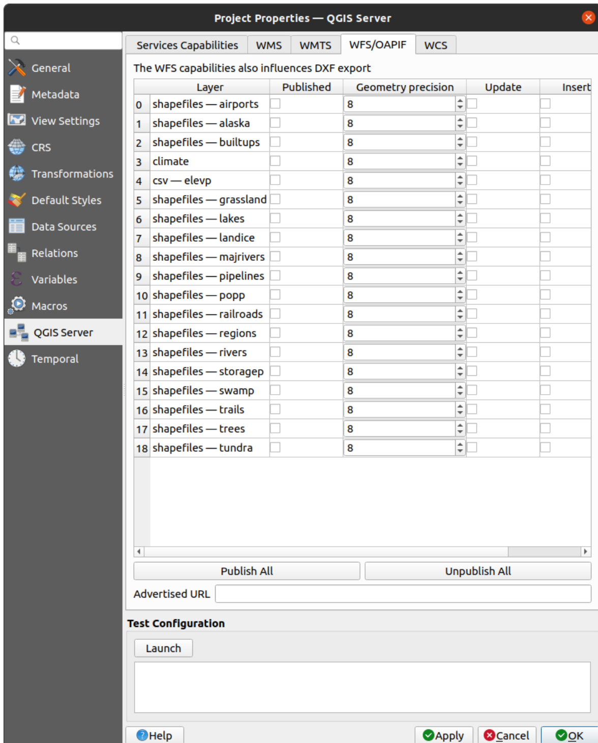
2.5 Fig. : Definitions in the WFS/OAPIF tab
