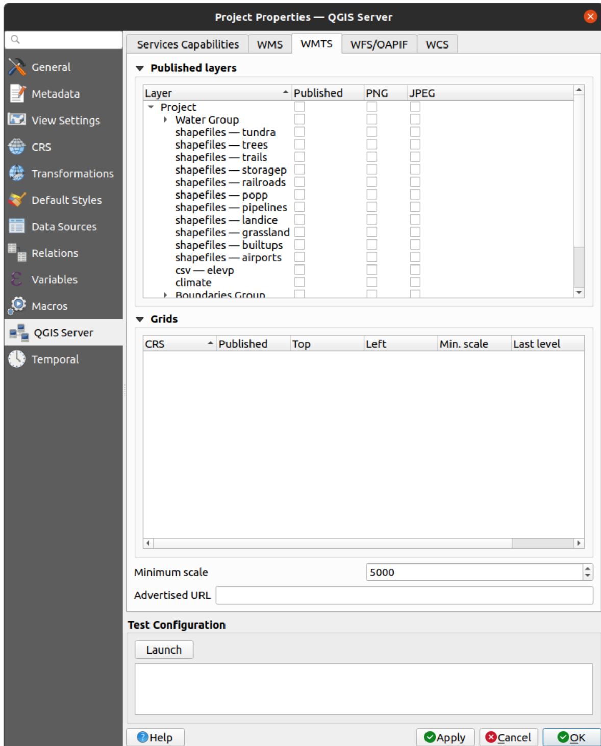
2.4 Fig. : Definitions in the WMTS tab
