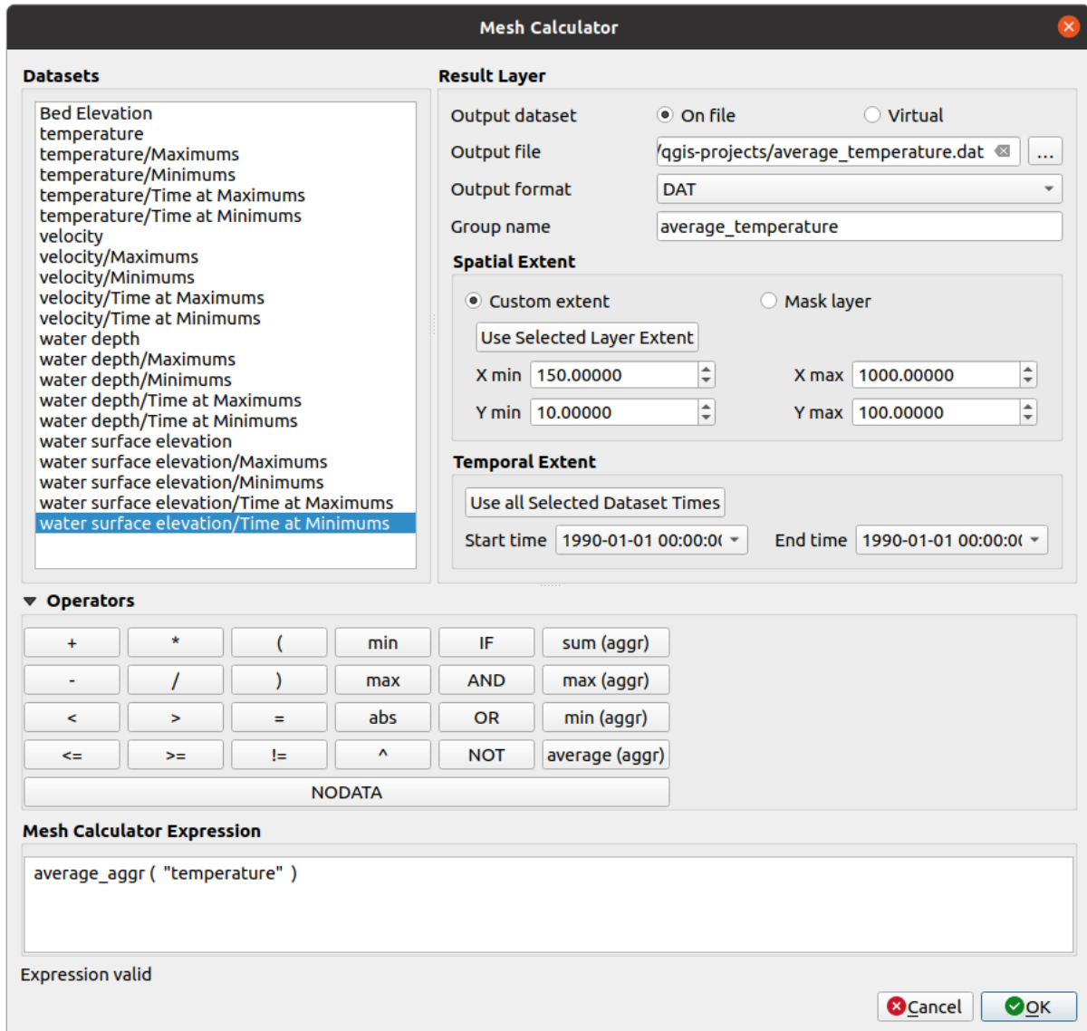
☒ 18.16 : Mesh Calculator
