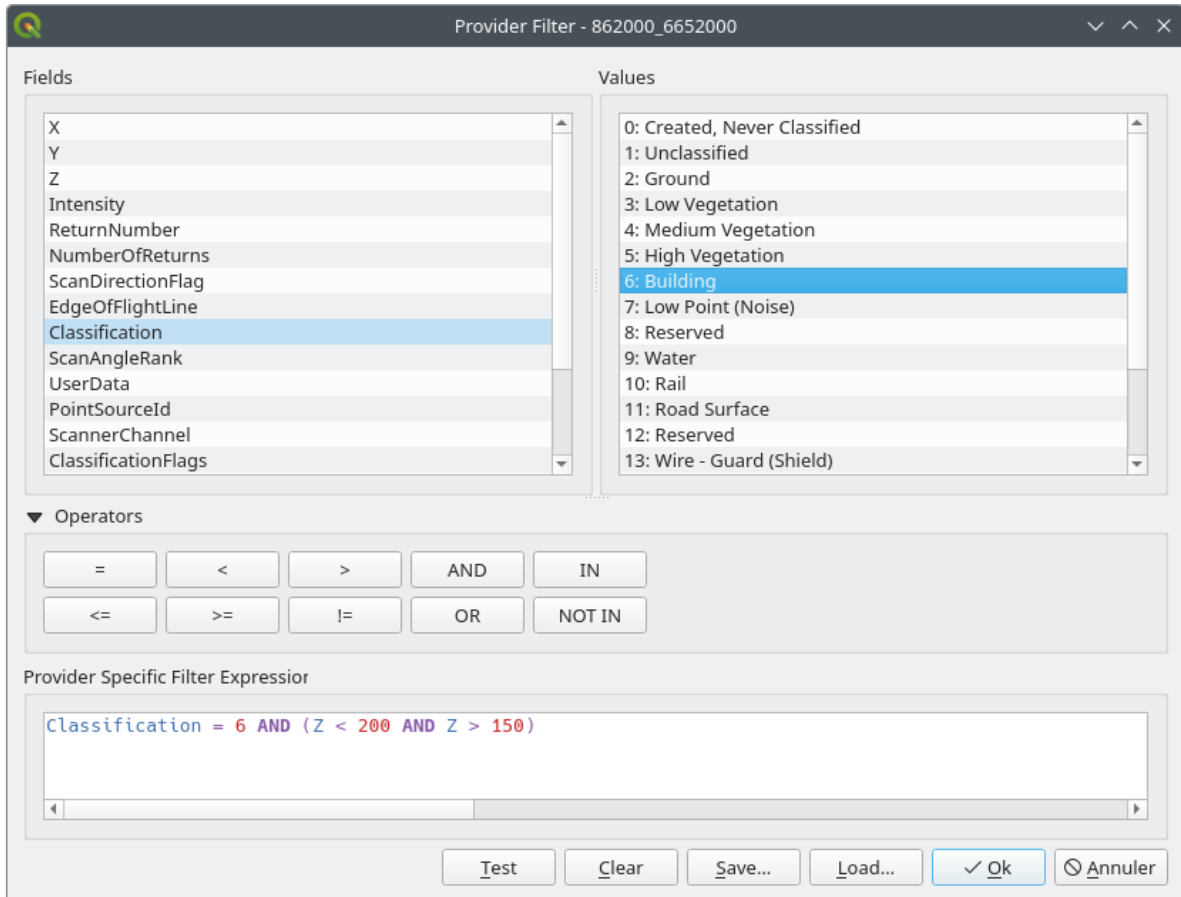
20.3. ábra: Filtering point cloud layer to buildings at specific altitude
