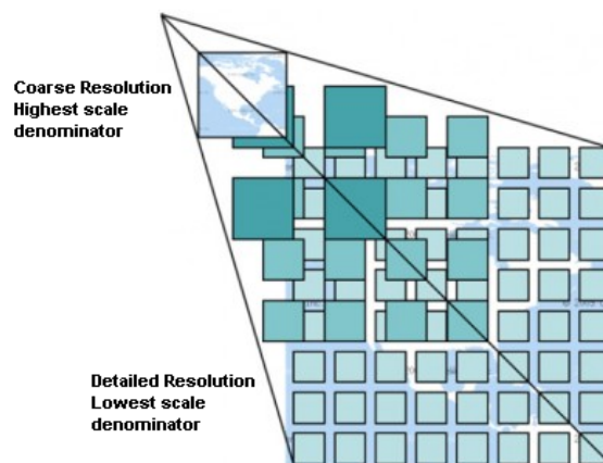
23.1. ábra: Concept of WMTS tile sets
