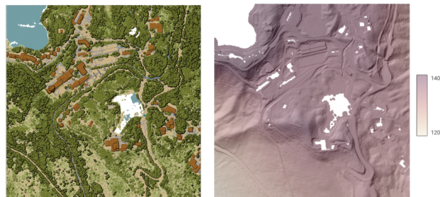
28.11. ábra: Terrain raster output generated by point cloud triangulation
