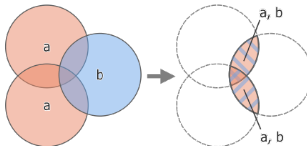
Figure28.123: Intersection operation between a two-feature input layer “a” and a single feature overlay layer “b” (left) - overlapping areas become a new two-feature layer with both layers’ attributes (right)
