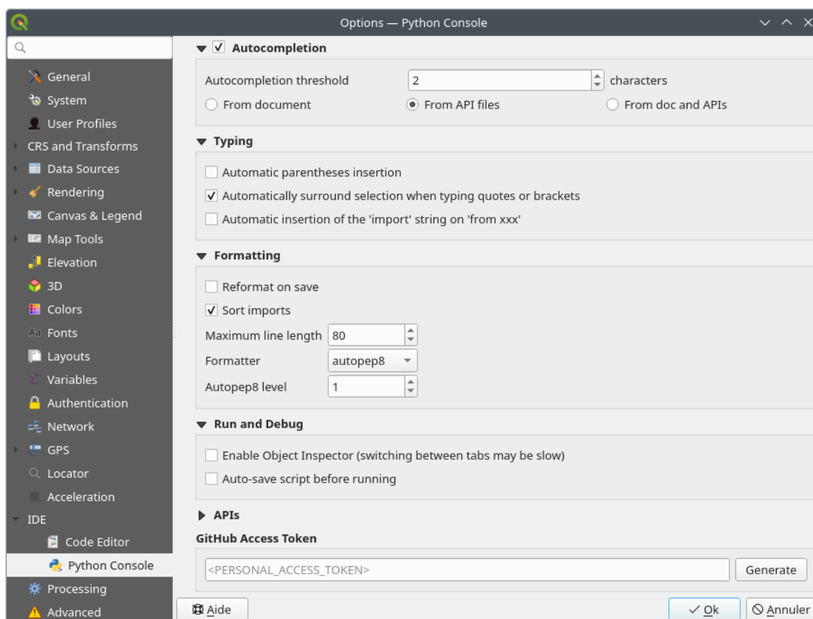
Abb. 9.28: Python Console settings
