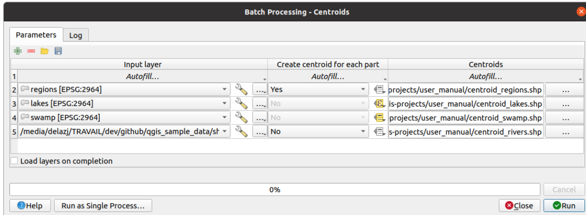
Abb. 27.34: Batch Processing
