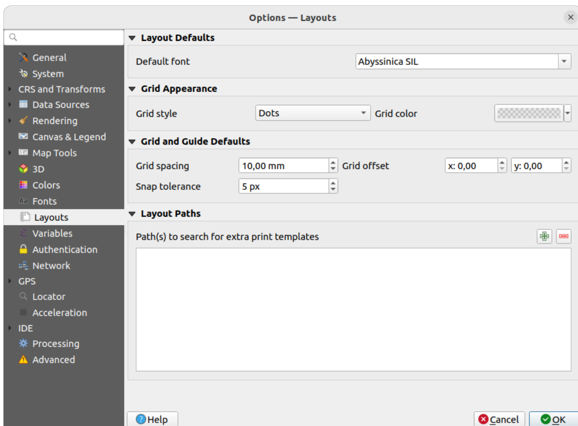
Abb. 9.20: Layouts settings
